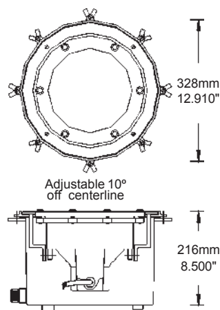
E600 A /-B69A Niche Mounting
