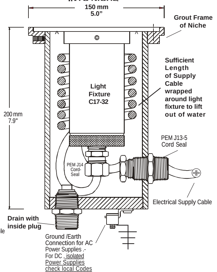
C 17-32 in Niche 0085 SIDE ELECTRICAL CABLE ENTRY INTO NICHE
