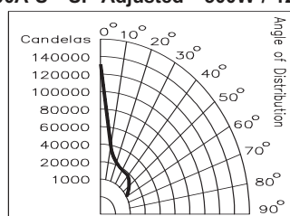
E300A-S - SP Adjusted - 500W / 120V
