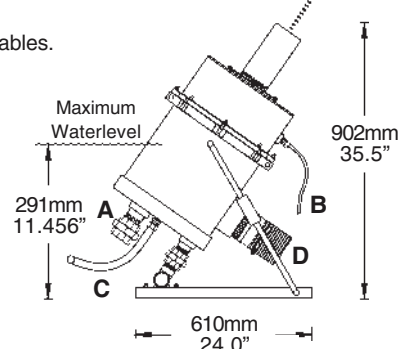
PEM 144M2 - 11 Jet assembly with Stand
